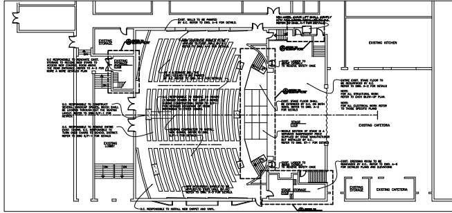
RENOVATION FLOOR PLAN
